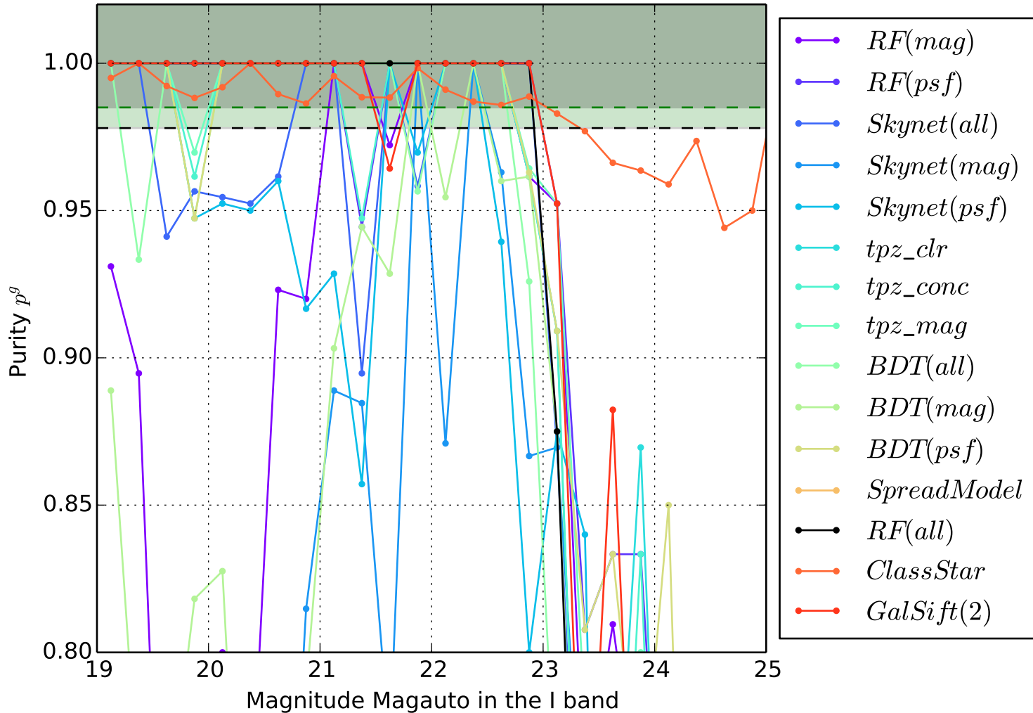
Purity p^s at c^s = 0.25 , for all classifiers
