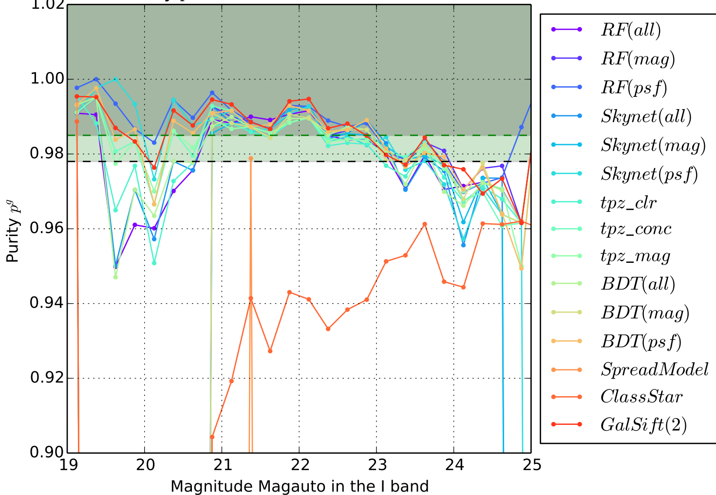
Purity p^g at c^g = 0.96 , for all classifiers
